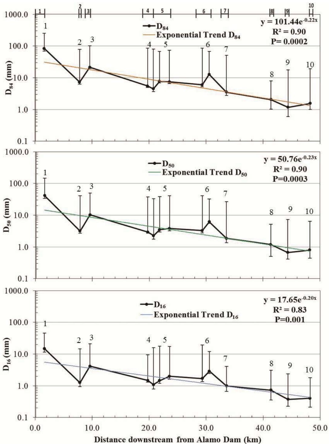
Figure 4. Log-average D_{16} , D_{50} and D_{84} , by reach, against distance downstream of Alamo Dam. The downstream trend is fit with an exponential equation for each size class. Vertical bars show the maximum and minimum D_{16} , D_{50} and D_{84} values within each reach.
