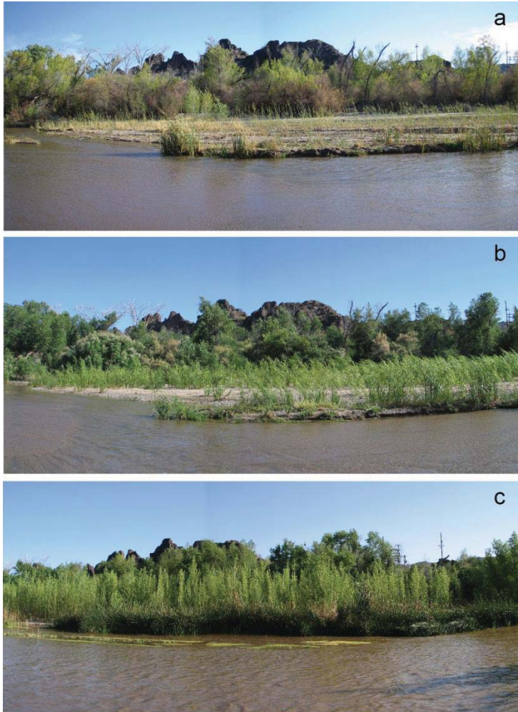
Figure 5. Repeat photographs of vegetation study bar in Mineral reach, looking from channel toward river left: (a) February 2006, (b) May 2006, (c) April 2007. Sequence illustrates growth of seedlings surviving floods and associated bar stabilization.
