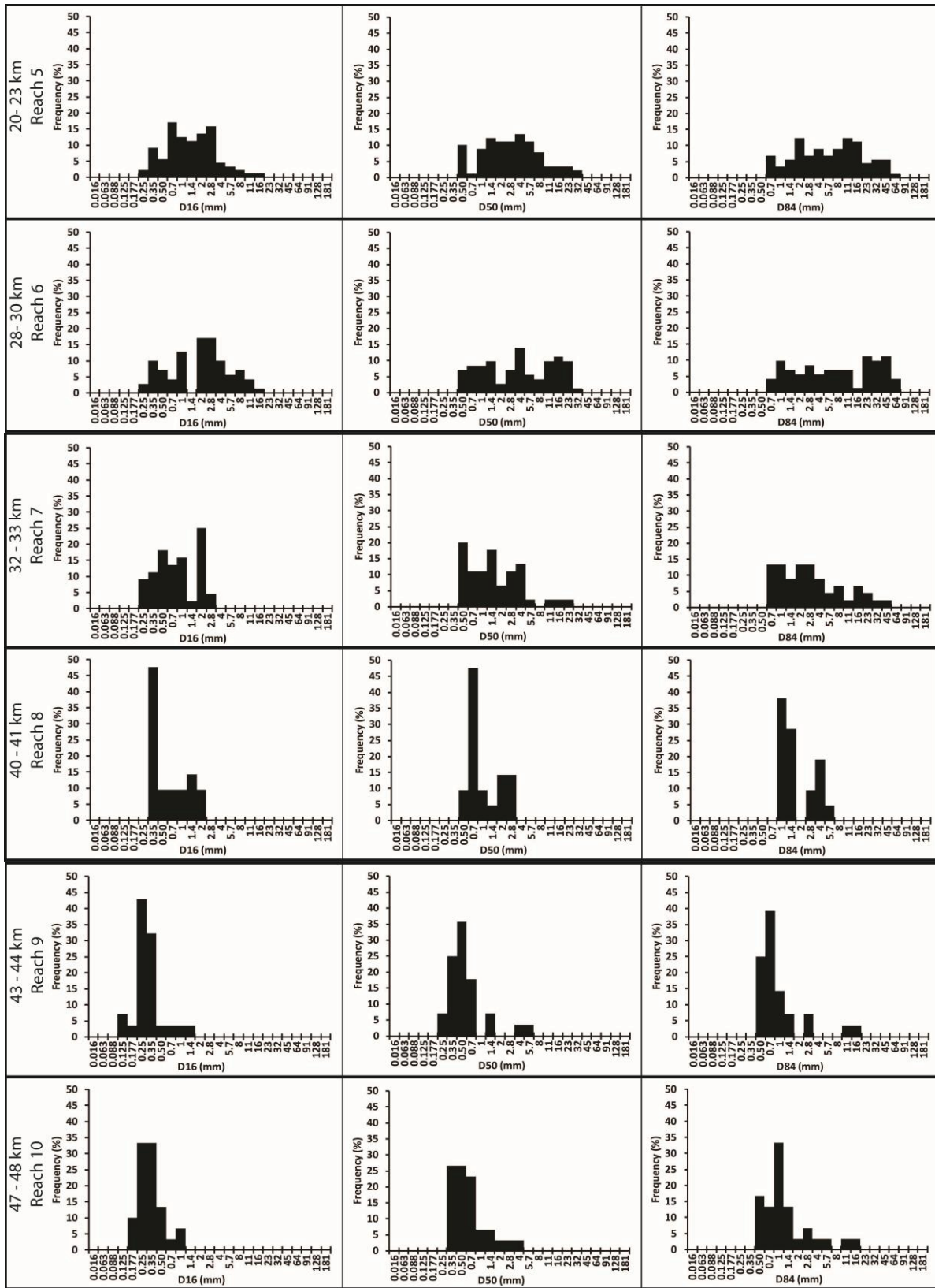
Figure D-5. Histograms with the frequency of D 16 , D 50 and D 84 grain sizes in each reach. Size is by half phi class.
