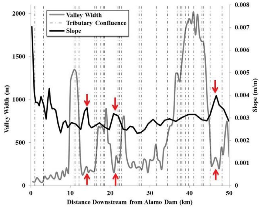
Figure D-4. Valley width and slope shown with distance downstream tributary confluence locations are represented by vertical dashed lines. Red arrows indicate areas of confinement that corresponded with increased slope.
