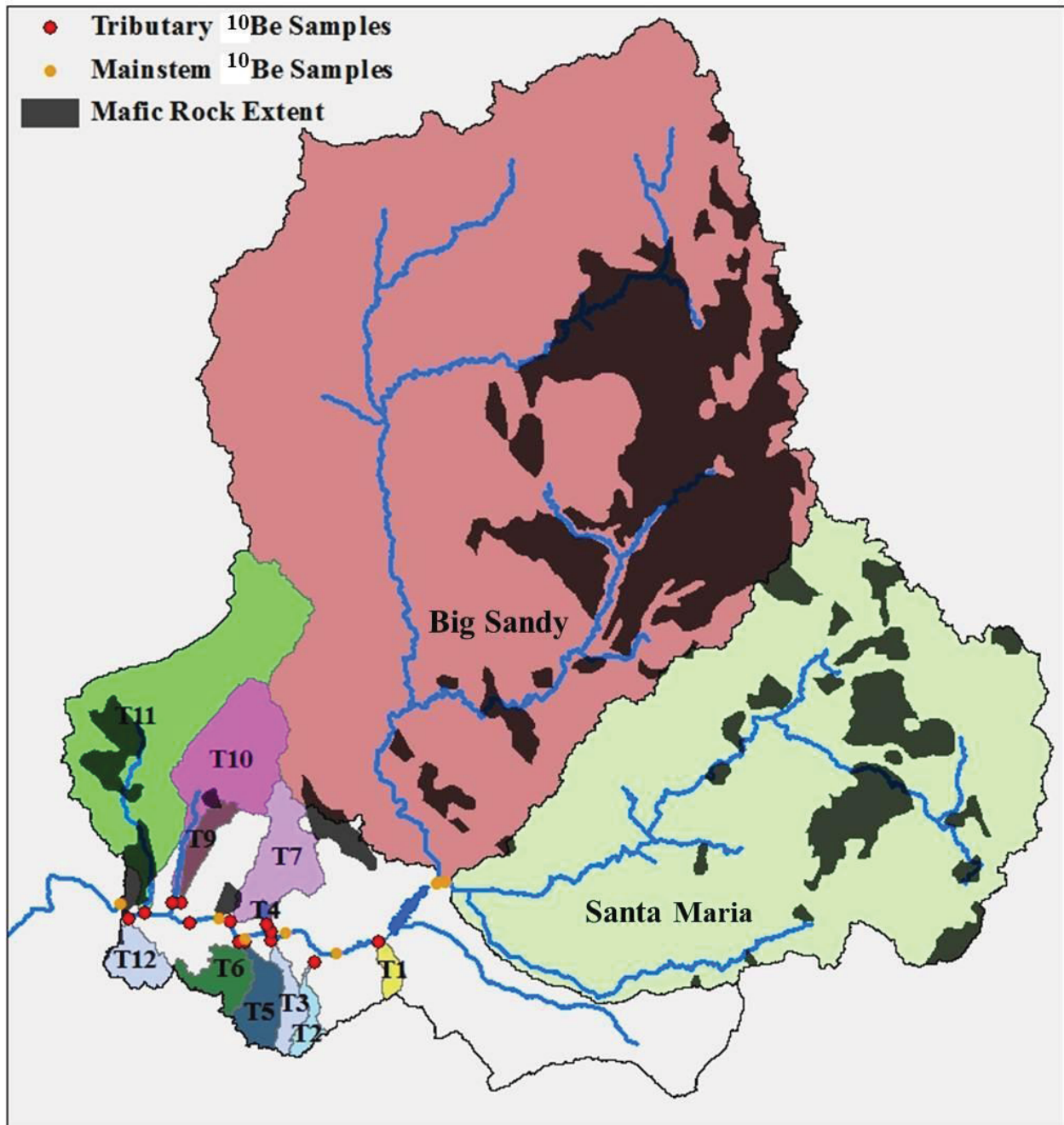
Figure B-1. The extent of mafic rock in the Bill Williams River watershed (Richard et al., 2000). A high percentage of mafic rock that is low in quartz could cause greater uncertainty in catchment nuclide concentration and erosion rate.
