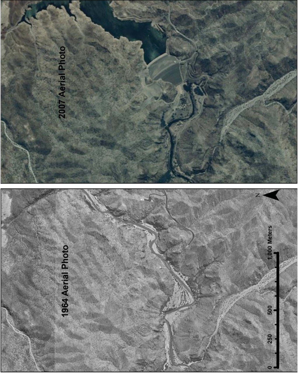
Figure E-2. Aerial photograph comparison of Bill Williams River at Alamo Dam site in 1964 and 2007.
