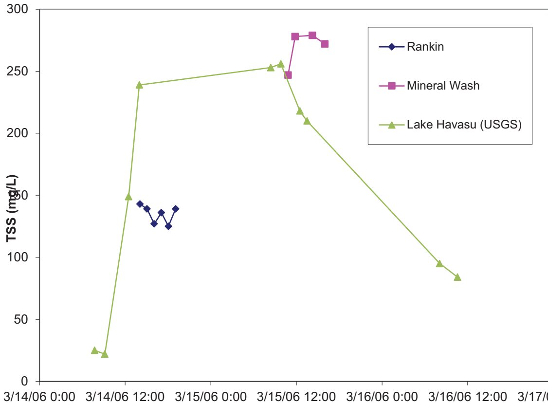
Figure 1-1. Suspended sediment transport measurements during March 2006 flood on Bill Williams River, including our measurements at Rankin and Mineral Wash and USGS measurements at the mouth of the BWR in Lake Havasu (Wiele et al., 2009).
