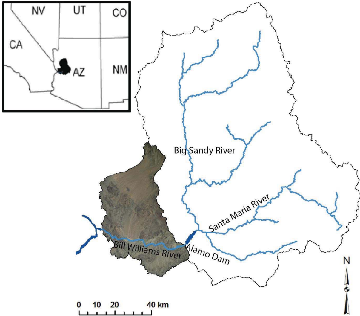
Figure 1. Bill Williams River basin. Inset map shows location in Arizona and southwestern United States. Large map shows BWR basin, with area downstream of Alamo Dam highlighted to show portion of basin that currently delivers sediment to mainstem BWR; supply from the upstream watershed area is cut off by the dam.
