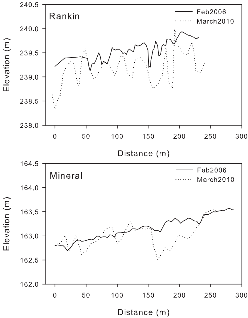
Figure 10: Longitudinal profiles of Rankin (top) and Mineral (bottom) study reaches at start (February 2006) and end (March 2010) of study period, where 0 on the x-axis is the downstream end of each study reach.
