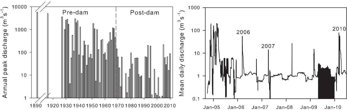
Figure 2. Flow data for the Bill Williams River below Alamo Dam gauge. Left panel shows annual peak discharges for the period of record and illustrates the post-dam reduction of high flows. Right panel shows mean daily flows from late 2004 to mid-2010, with annotations of flood events around which our data collection was completed; note difference in y-axis scale compared to left panel.
