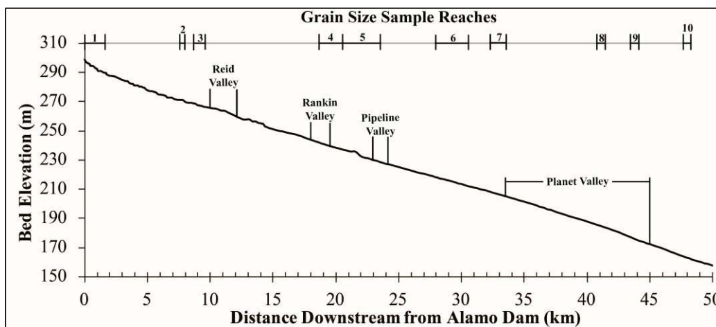
Figure 2. Longitudinal profile of the BWR downstream of Alamo Dam from US Army Corps of Engineers HEC-RAS modeling from 2006 3 m LIDAR data. Valleys >500 m wide and 10 reaches where grain size was sampled are labeled.
