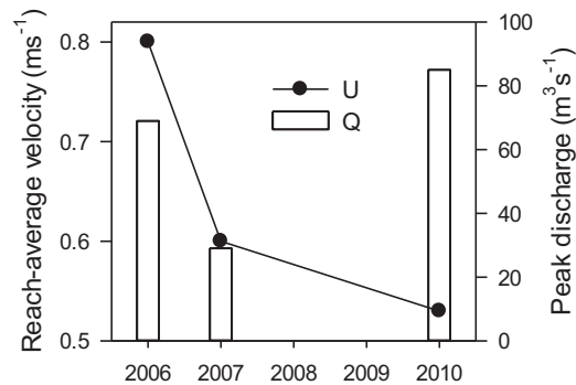
Figure 12. Velocities averaged over the 18-km reach from Alamo Dam to the Rankin reach, based on the time between flow releases at Alamo (from USGS gauge data) and their arrival at Rankin (from pressure transducer and/or visual records); right axis shows corresponding peak discharges released at Alamo. The pattern reflects increasing vegetation drag.
