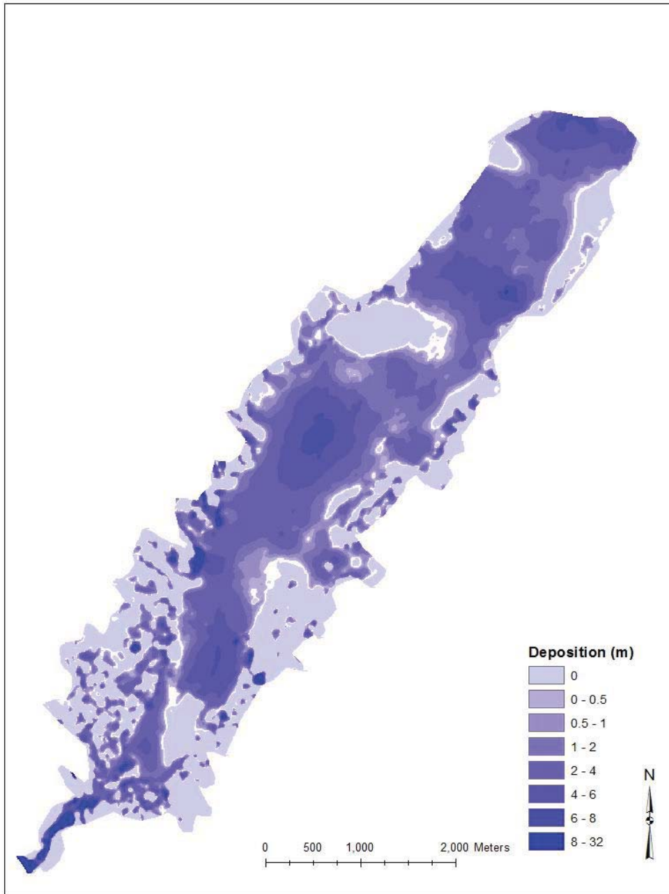
Figure C-1. Sediment deposition in Alamo Lake between 1968 and 1985 found by comparison of digital elevation models (DEMs) (US Army Corp of Engineers, 1963; US Army Corp of Engineers, 1985). Erosion rate found from the total deposition in those 17 years was 270 \pm 20 \text{ t/km}^2/\text{yr} . This is greater than the long-term rates of erosion found from cosmogenic nuclide analysis.
