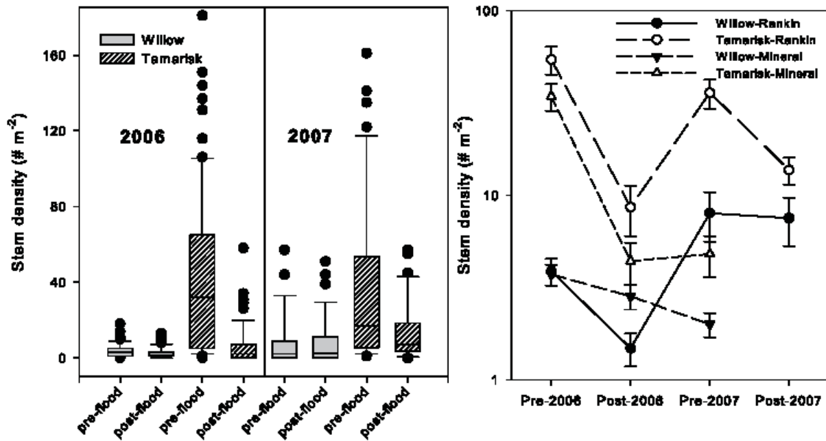
Figure 6. Stem densities of willow and tamarisk before and after 2006 and 2007 floods. Left panel shows distributions of measured densities, with 2006 data from Rankin and Mineral combined and 2007 data from Rankin only (boxes bound 25 th and 75 th percentiles, solid lines in boxes illustrate medians, and whiskers bound 10 th and 90 th percentiles). Right panel shows mean and standard error of stem densities, differentiated among species and reaches. Densities for post-2007 in Mineral were not measured because the 2007 event did not inundate vegetation plots in that reach.
