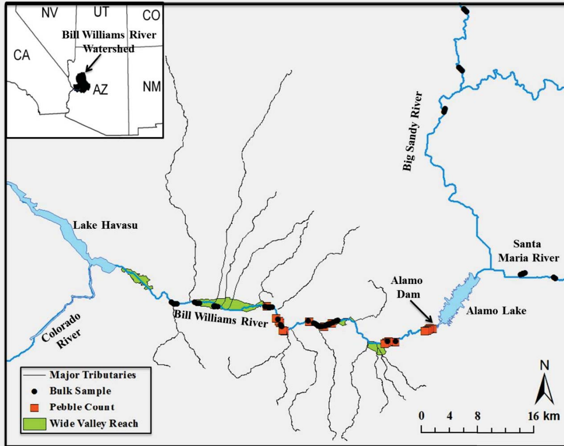
Figure 1. The Bill Williams River watershed in Arizona, USA (upper left) and sediment sample locations. Photo grain size locations overlap with the bulk samples and pebble counts at 30m intervals, but are not shown. Valley reaches with widths >500m are shown in green. Tributaries downstream of Alamo Dam with greater than >20km 2 catchment areas are marked with black lines.
