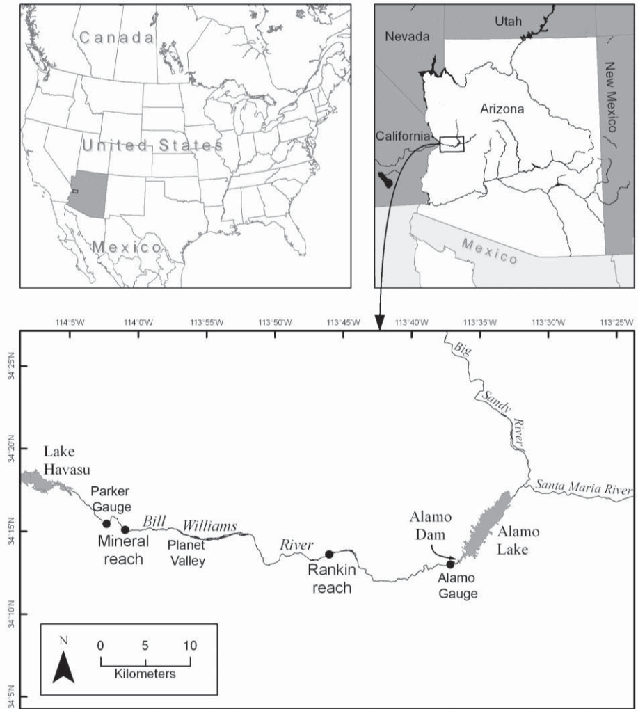
Figure 1. Bill Williams River in western Arizona, USA. The two study reaches identified in the bottom panel, Rankin and Mineral Wash, are 18 and 48 km downstream of Alamo Dam, respectively (flow is from right to left).
