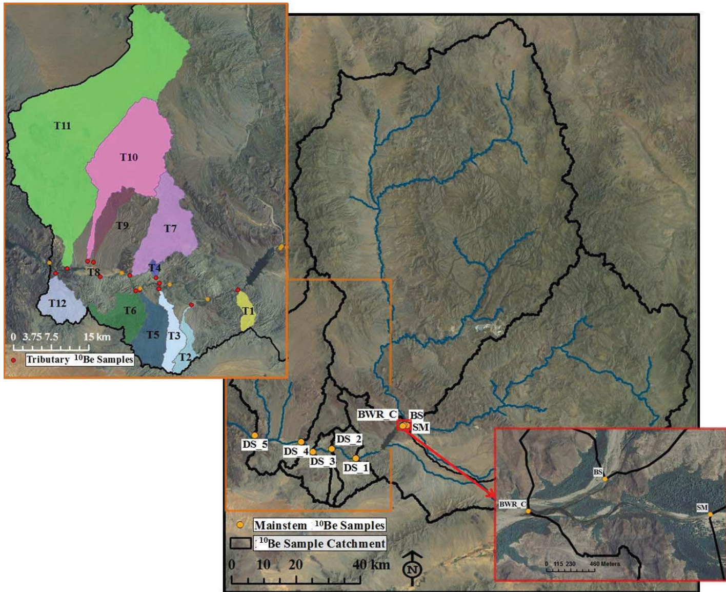
Figure 1. Sample locations for cosmogenic nuclide analysis in the BWR watershed. Samples BS, SM, and BWR_C (lower right inset) were upstream of Alamo Dam. All other samples were from downstream of the dam, including DS_1 – 5 (mainstem BWR) and T1 – 12 (tributaries; upper left inset).
