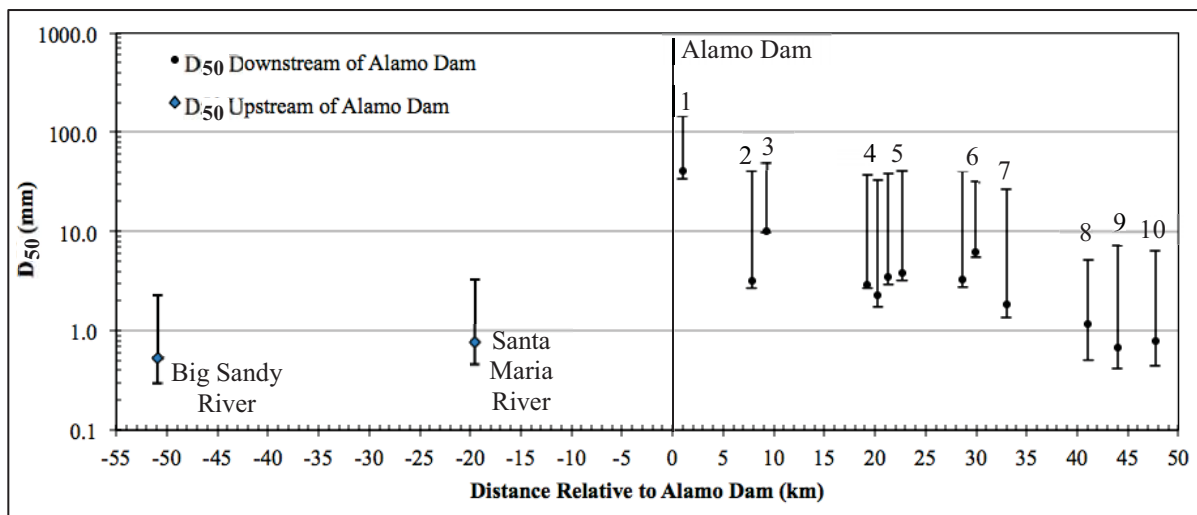
Figure 3. Log-average D_{50} for each reach, with error bars showing the maximum and minimum D_{50} in each reach. Comparison of reaches upstream and downstream of Alamo Dam shows a large increase in grain size, with downstream fining below the dam.
