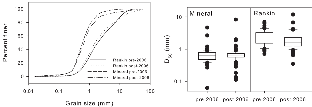
Figure 11. Grain size data from Rankin and Mineral before and after 2006 flood: left panel shows size distributions of composited bulk samples, and right panel shows median grain size ( D_{50} ) for all samples.
