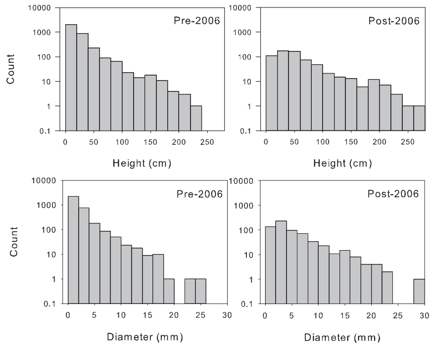
Figure 8. Histograms of plant heights (top) and diameters (bottom) measured in February and May 2006, before and after the 2006 flood, with reaches (Mineral and Rankin) and species (tamarisk and willow) combined. Data are based on repeat measurements of the same study plots. The histograms illustrate size-dependent mortality during the 2006 flood, primarily occurring among plants <40 cm in height and <4mm diameter.
