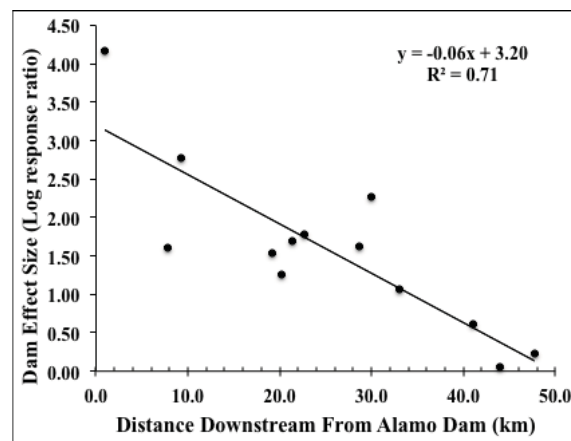
Figure 5. Dam effect size as a log response ratio with distance downstream from Alamo Dam. The dam effect size is greatest near Alamo Dam and decreases linearly downstream.
