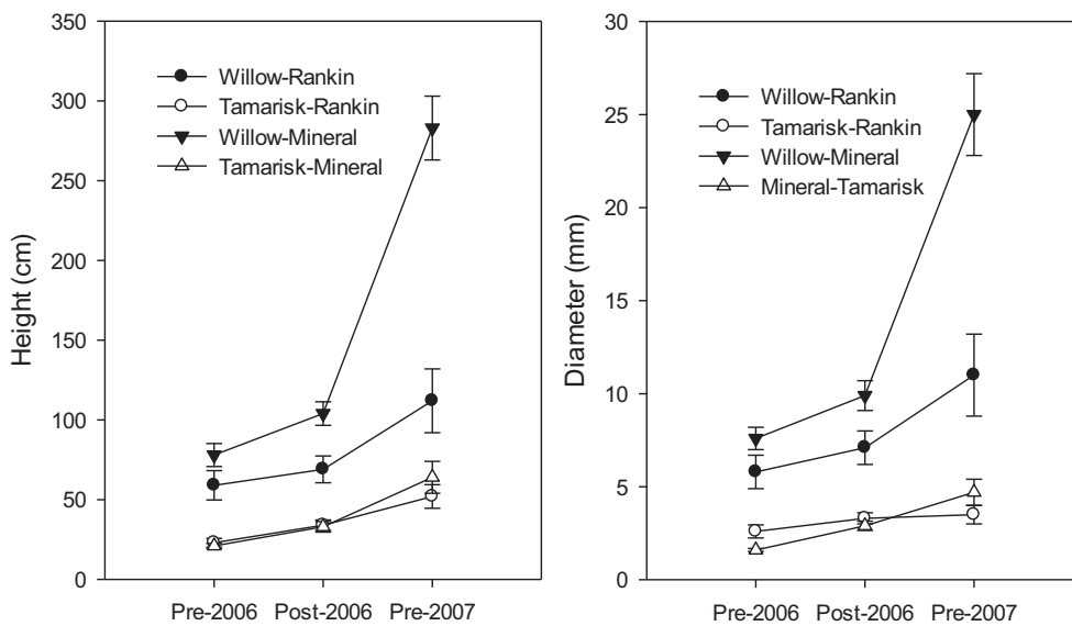
Figure 7. Seedling height and diameter (mean and standard error) measured in February 2006 (pre-flood), May 2006 (post-flood) and April 2007 (pre-flood), for willow and tamarisk, in Rankin and Mineral study reaches. Because vegetation measurements following the 2007 event were taken within one week of the pre-flood measurements, a time period in which minimal plant growth would have occurred, diameter and height were not measured after the 2007 event.
