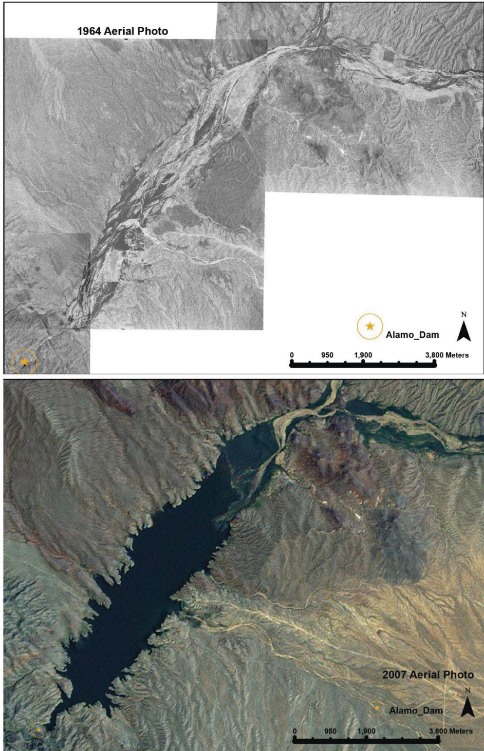
Figure E-1. Aerial photograph comparison of Alamo Valley (1964) and Alamo Reservoir (2007).
