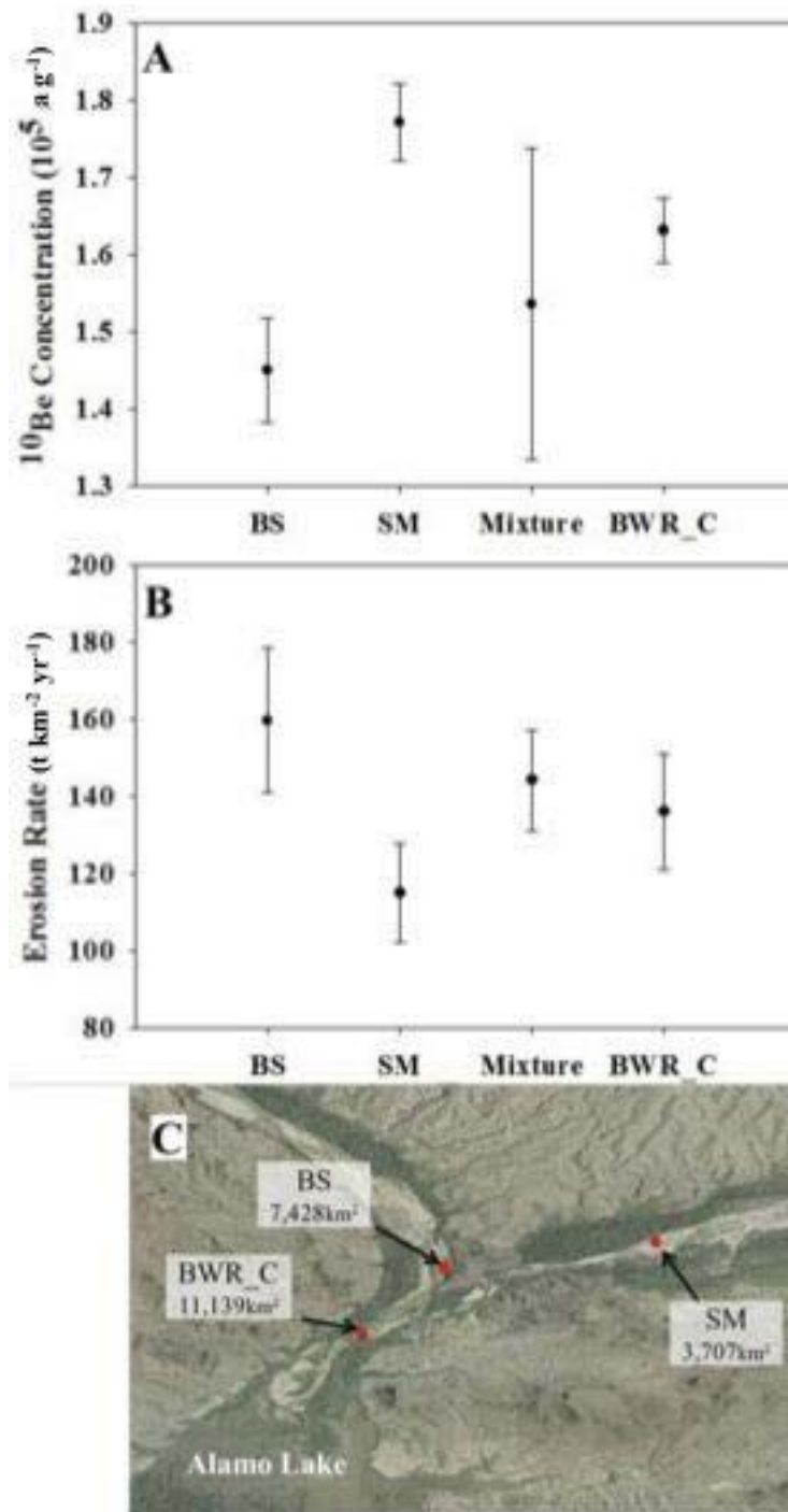
Figure 3. Comparison of results from measured samples in Big Sandy (BS), Santa Maria (SM) and BWR_C with results of calculations of BS and SM sediment mixing (Mixture), expressed in terms of ^{10}\text{Be} concentrations (A) and erosion rate (B). Locations of BS, SM and BWR_C samples are shown in (C) and in Figure 1. Mixture results are near the BWR_C values, which indicates BS and SM are well mixed in the BWR_C sample. Error bars show value uncertainty, and the mixing calculation result is a propagated uncertainty.
