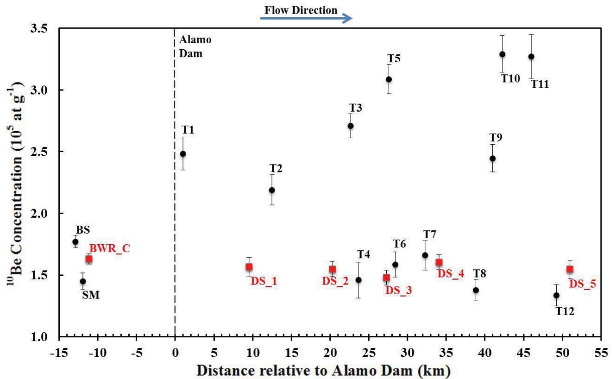
Figure 2. Nuclide concentration results versus distance relative to Alamo Dam. Error bars are from analytical error to determine ^{10}\text{Be} concentration. Below-dam mainstem concentrations were similar to above-dam samples; tributaries show variable nuclide concentration.
