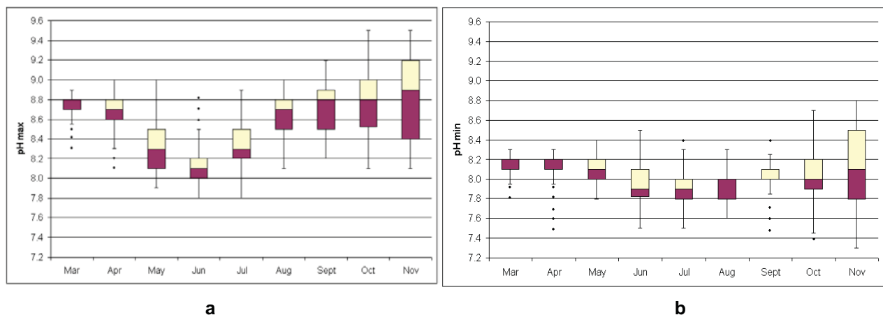
Figure 6. Box plots of monthly maximum (a) and minimum (b) pH values for the Snake River at Moose, Wyoming, for the period of record (2002–2008).
