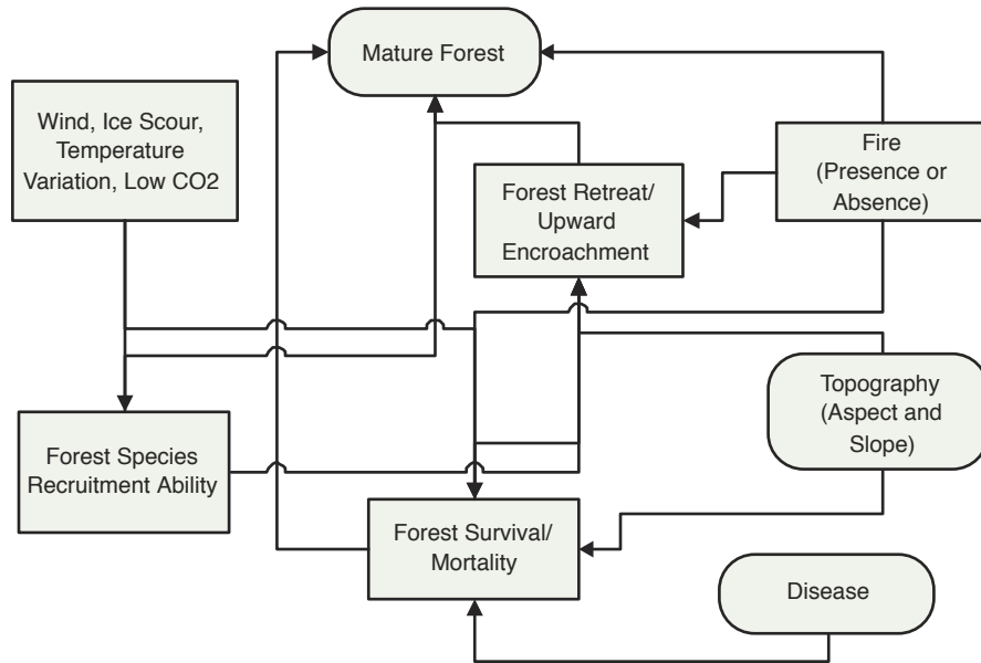
FIGURE 8 Alpine timberline elevation submodel.
