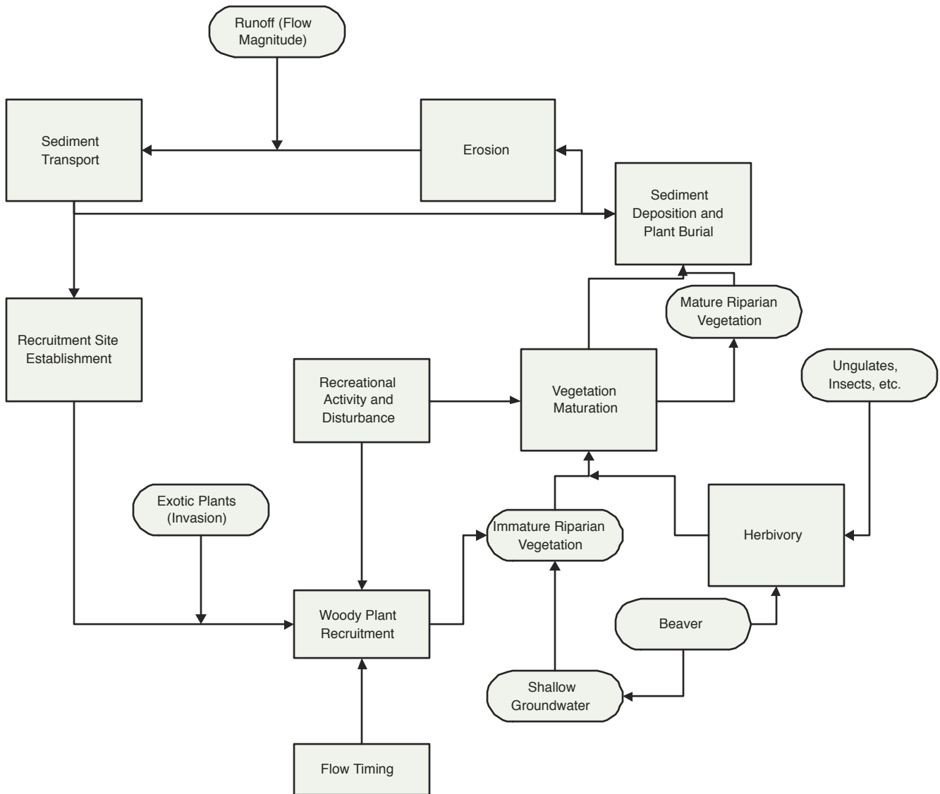
FIGURE 26 Riparian vegetation dynamics submodel.
