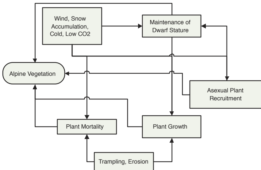
FIGURE 6 Alpine vegetation submodel.
