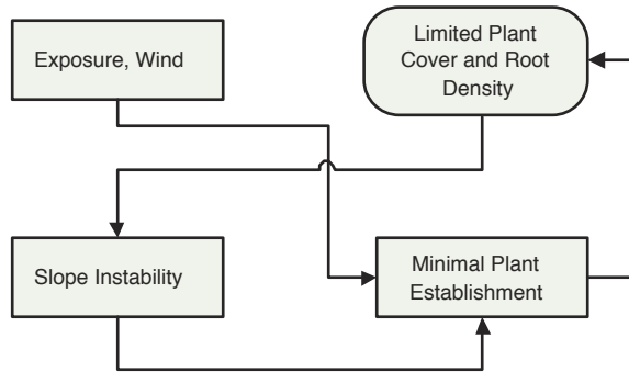
FIGURE 5 Alpine scree slope dynamics submoel.
