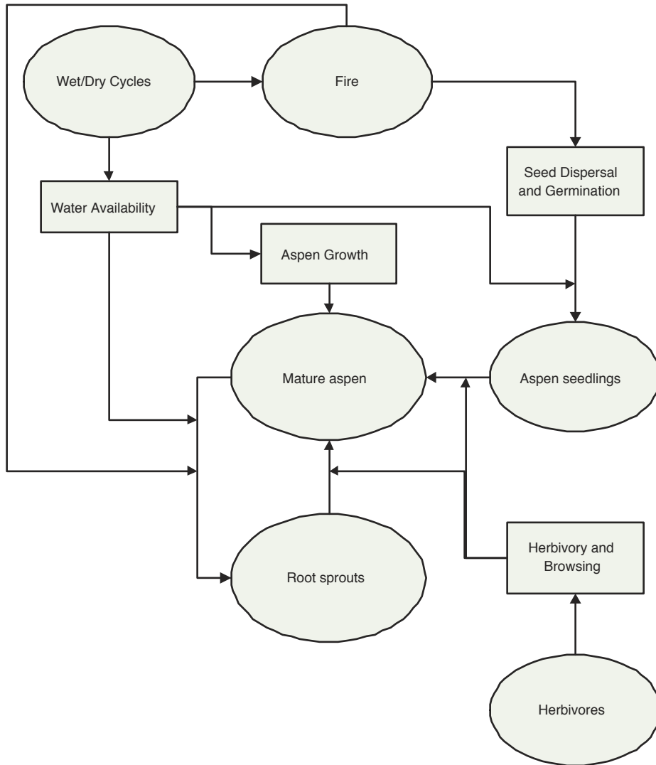
FIGURE 11 Aspen growth and reproduction submodel.
