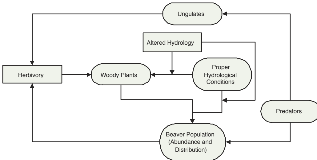
FIGURE 32 Wetland beaver population dynamics submodel.
