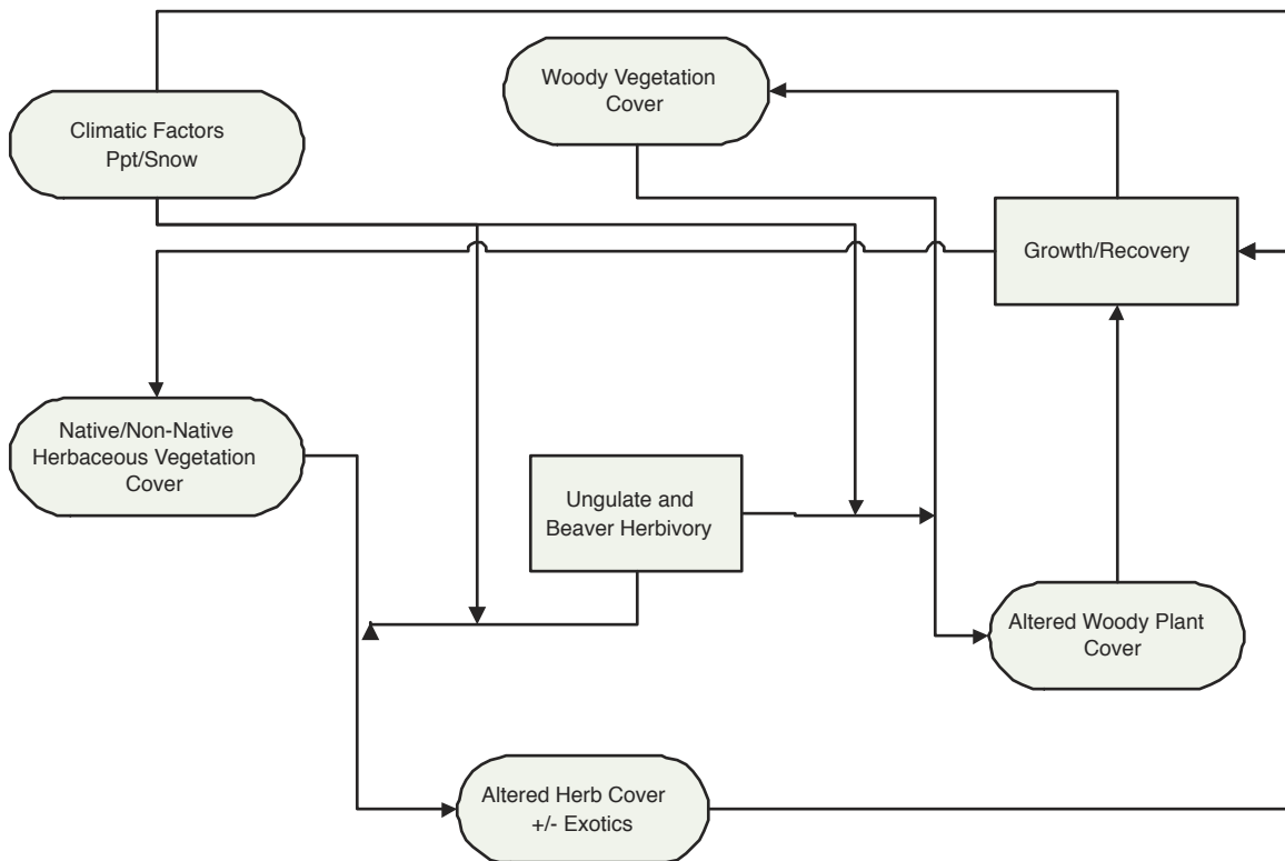
FIGURE 28 Riparian herbivory dynamics model.
