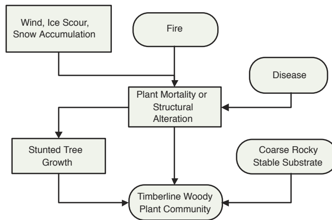
FIGURE 9 Alpine woody vegetation dynamics model.
