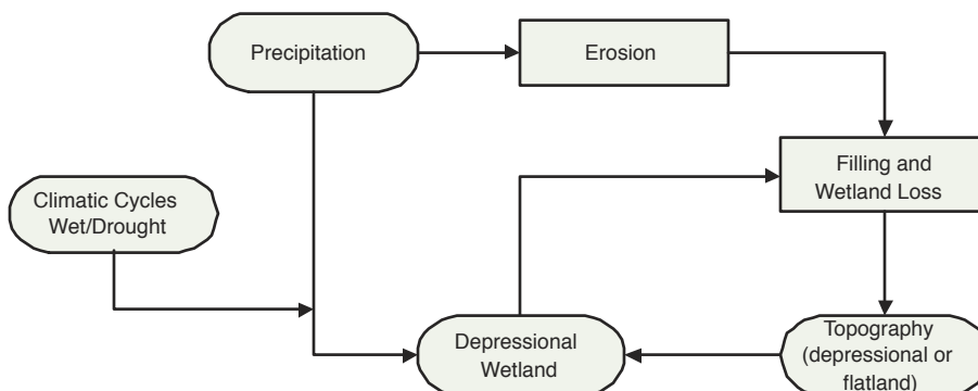
FIGURE 33 Depressional wetland dynamics submodel.
