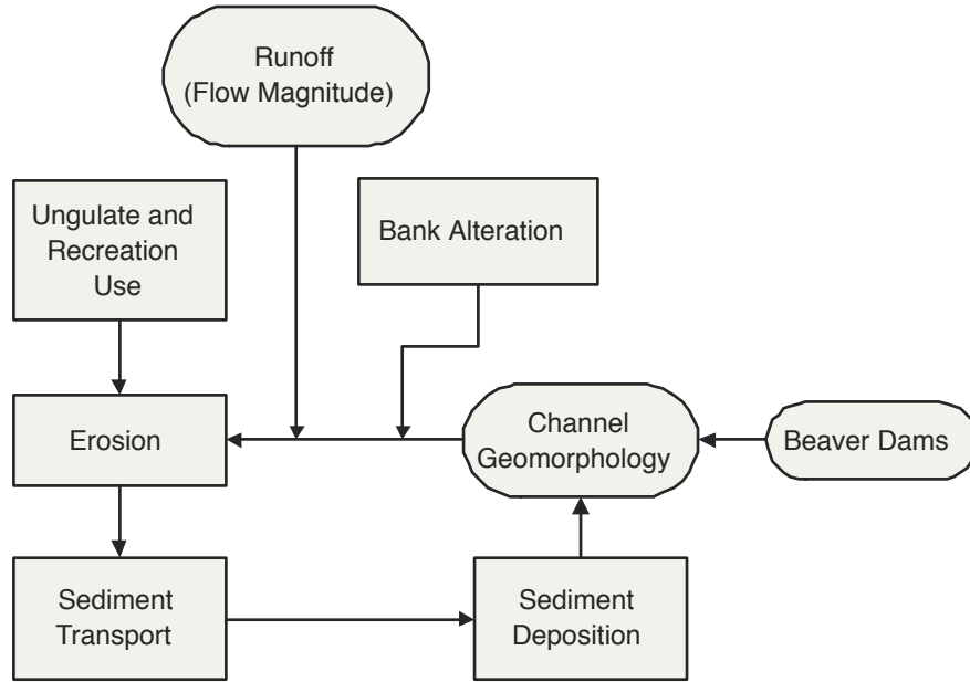
FIGURE 27 Riparian fluvial geomorphology dynamics submodel.
