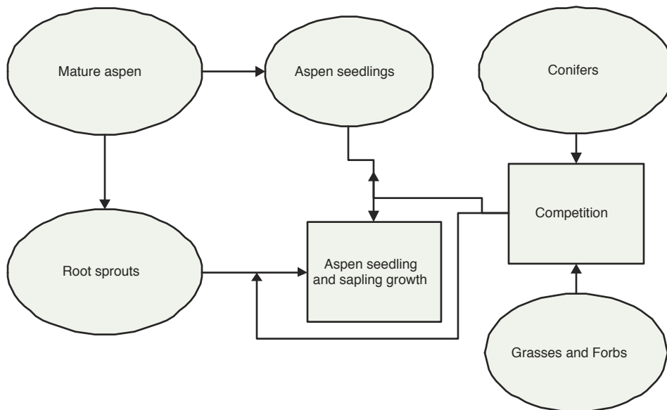
FIGURE I4 Aspen vegetarian composition submoel.
