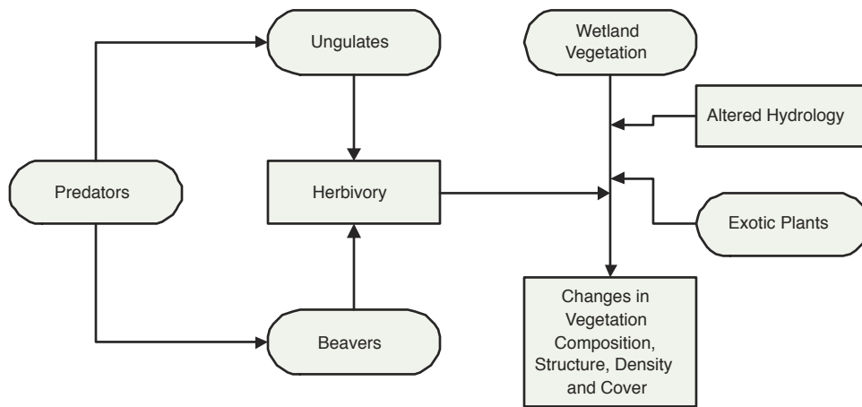
FIGURE 31 Wetland vegetation dynamics submodel.
