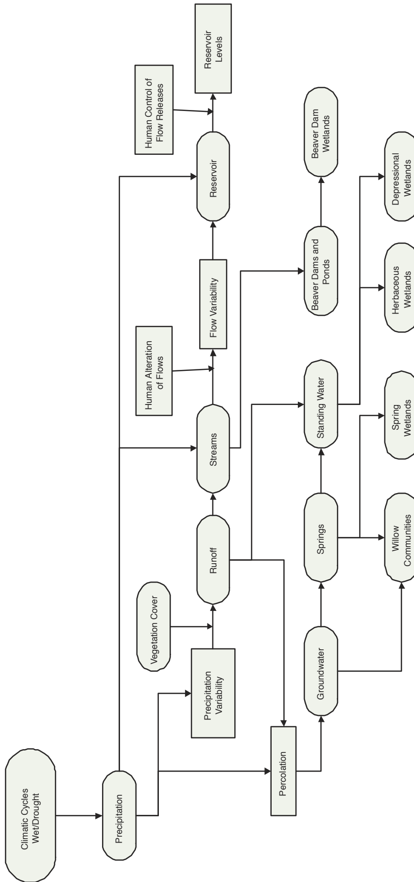
FIGURE 30 Wetland hydrology dynamics submodel.
