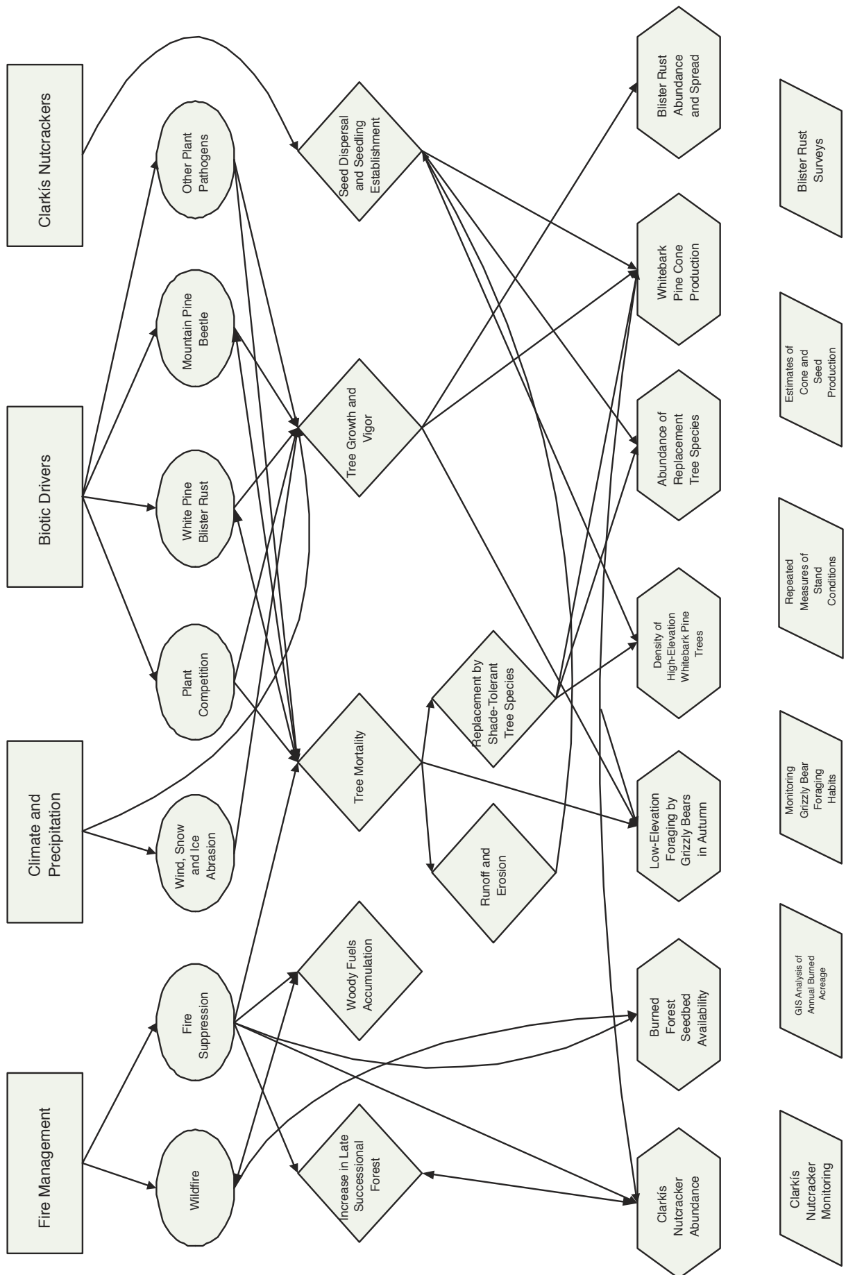
FIGURE 24 Whitebark pine model.
