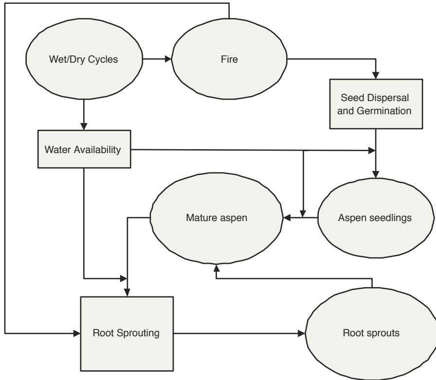
FIGURE I3 Aspen fire dynamics submoel.
