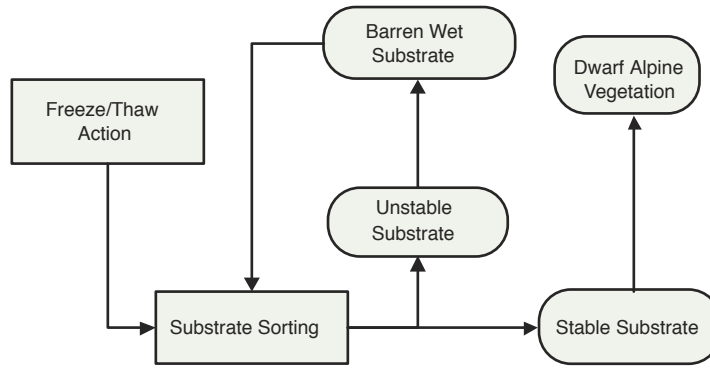
FIGURE 4 Alpine soil frost dynamics submoel.
