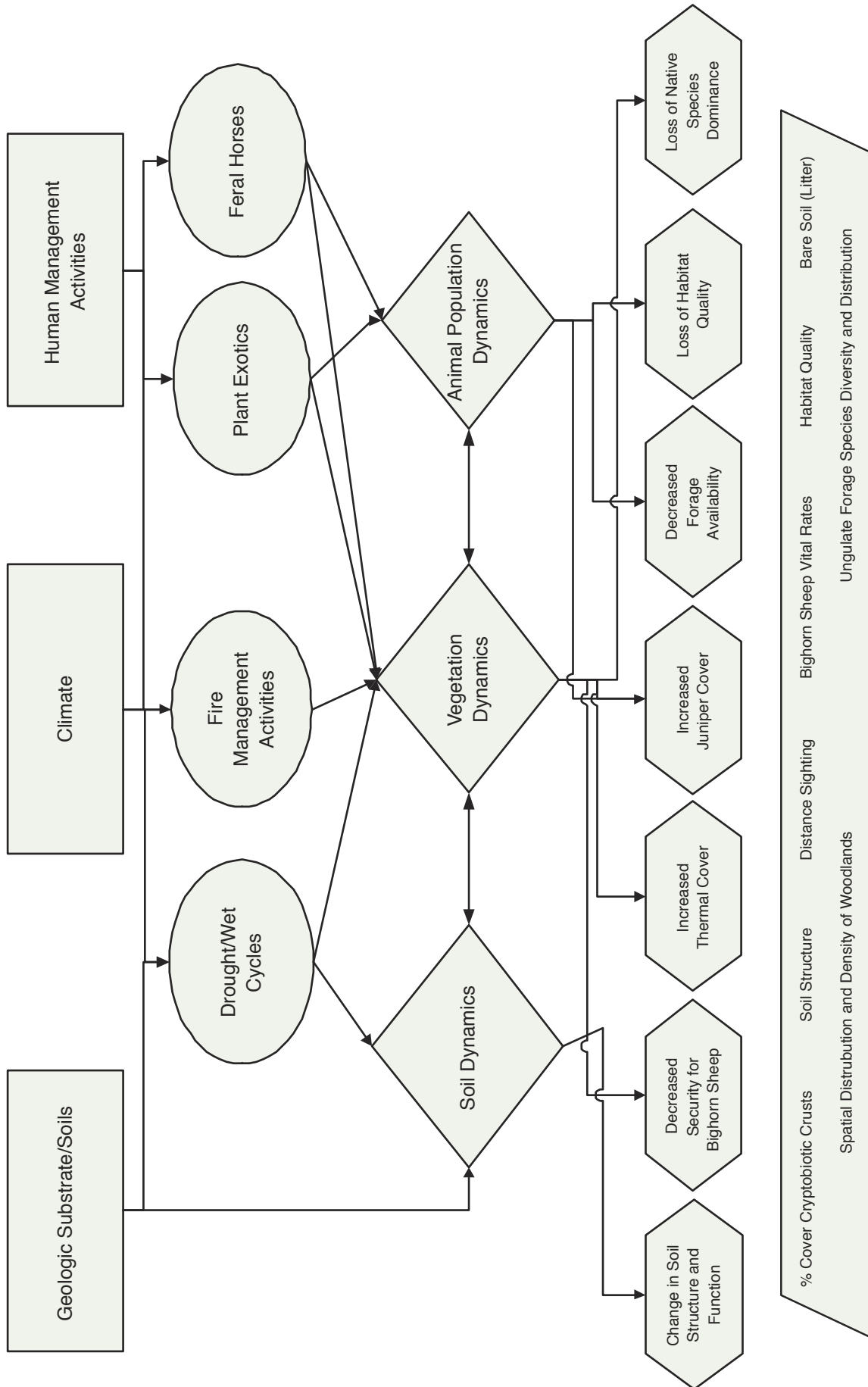
FIGURE 16 Dry woodland model.
