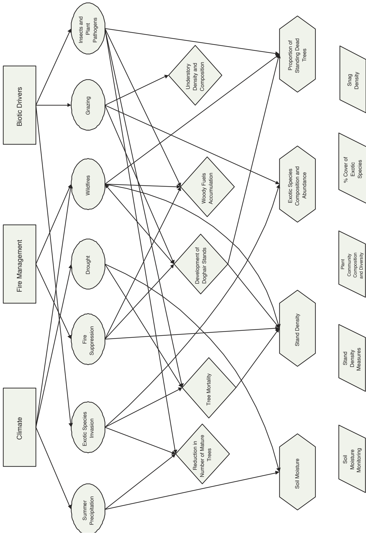
FIGURE 23 Ponderosa pine model.
