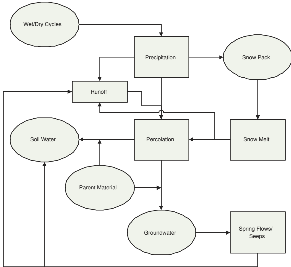
FIGURE I 2 Aspen soil and groundwater processes submodel.
