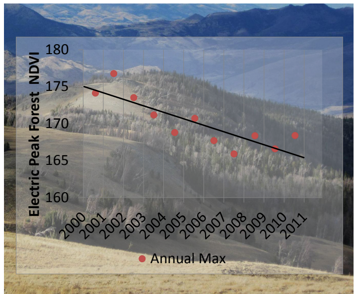
Graph indicating a decrease in NDVI related to tree die off.
