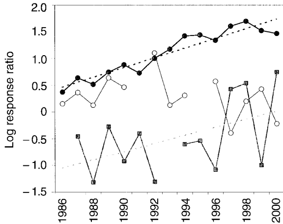
Fig. 2. Time series of the log response ratio between the exclusion treatment ( X_c , low-wolf area) and control ( X_c , high-wolf area) for elk density (solid circles), spring calf:cow recruitment ratio (open circles), and wolf kill rate of elk (gray squares) in Banff National Park from 1986 to 2000. Dashed lines represent general linear regression trends during the study, and missing values are indicated by breaks. There was no significant trend in calf:cow ratio, indicating stationary trophic effects of wolves on calf:cow ratio. Log response ratio values above zero represent higher responses in the partial wolf-exclusion area, X_c (i.e., higher elk densities), whereas values below zero represent higher responses in the control area, X_c (i.e., higher wolf kill rates).
