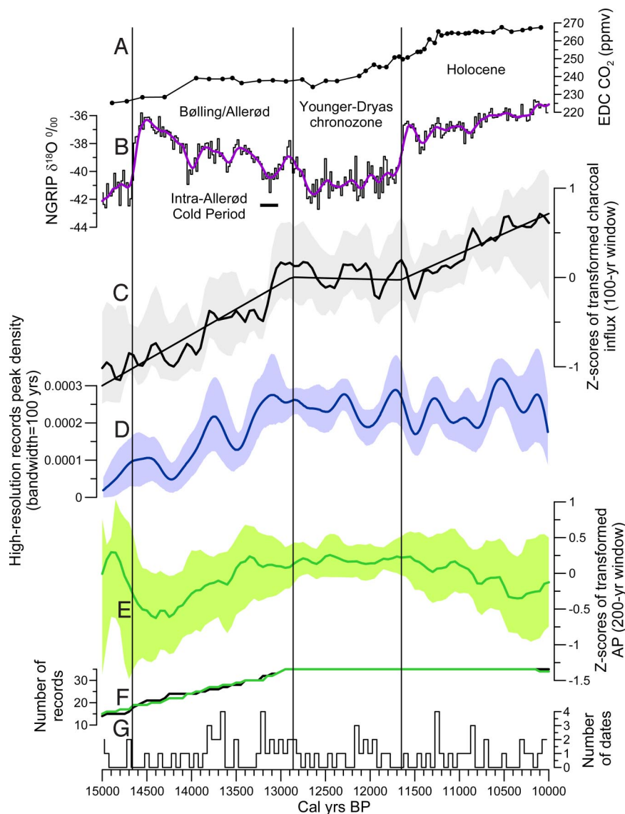
Fig. 1. Reconstructions of biomass burned, fire frequency, and woody biomass levels in North America. (A) The CO 2 ice-core record from Antarctica (41). (B) The NGRIP \delta^{18}\text{O}_{\text{ice}} record, a proxy for North Atlantic temperatures (21). (C) Reconstruction of biomass burned based on 35 records; the straight lines are segmented regression curves, and the smooth curves are local-regression fitted values. (D) Reconstruction of fire frequency based on 15 high-resolution records, expressed as the density of peaks per site-year. (E) Trends in woody biomass based on 35 records. (F) Number of records contributing to the biomass burning (black) and woody biomass (green) trends. (G) Number of dates per 50-year interval in the 35 paleo records. Confidence intervals (95%) are based on bootstrap resampling of sites. Vertical lines mark the beginning ( \approx 12.9 ka) and ending ( \approx 11.7 ka) of the YDC.
