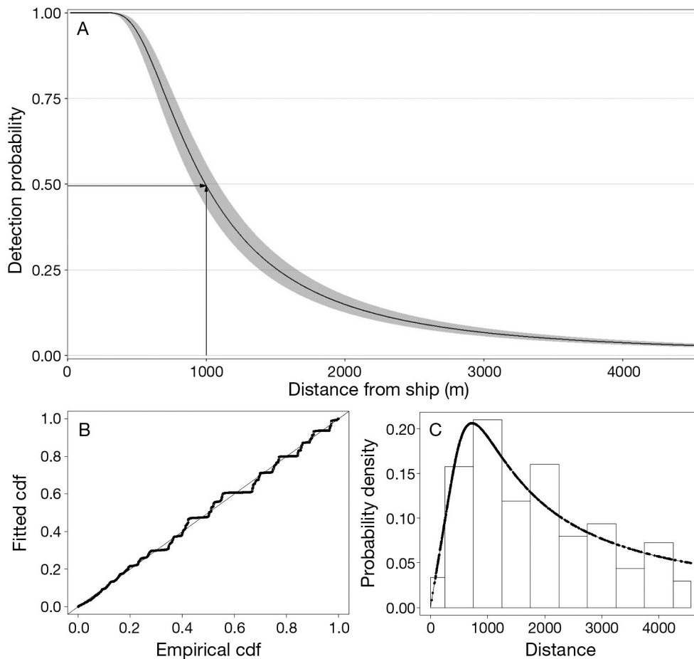
Fig. 4. Detection probability as it varies with distance (range = 0 to 4565 m) between ships and whales in and near Glacier Bay National Park from 2008 to 2015 (N = 3262). (A) Detection function. Shaded area around line indicates 95% confidence intervals. Arrows identify detection probability at 1000 m reference distance. (B) Quantile-quantile (Q-Q) plot. (C) Probability density function over radial first sighting distances binned in 10 distance classes. cdf: cumulative distribution function
